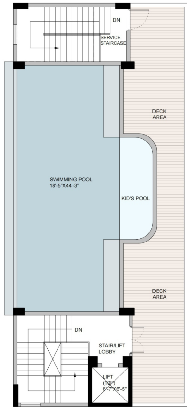
ROOF TOP PLAN
